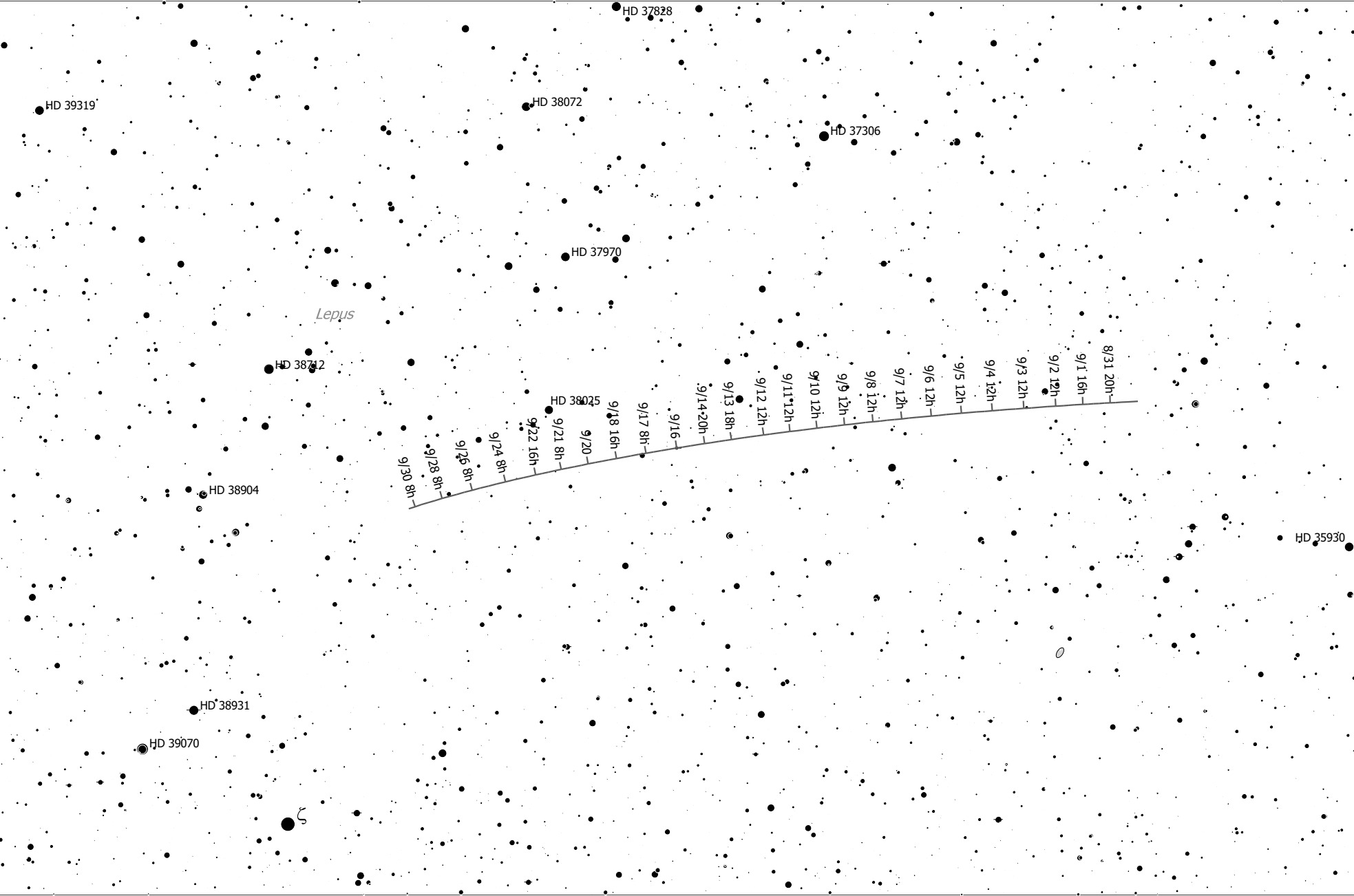
C/2024 T5 (ATLAS) (Comet) Magnitude: 13.74 Coma Diameter: 46" SBr: 21.8 Mag/arcsec² Earth Distance: 4.2 AU
